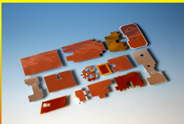
Preinsulated die cut pieces of copper, tin clad copper or aluminium
